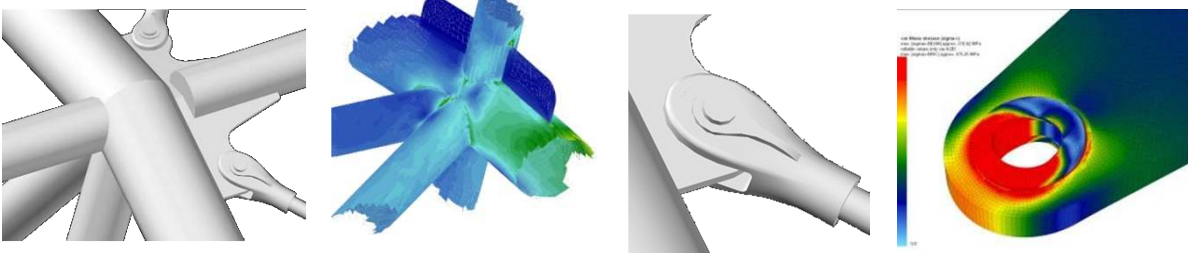
Fig. 7 CAD visualization, shell nad bricks FEM model a) typical node, b) connection of bracing
