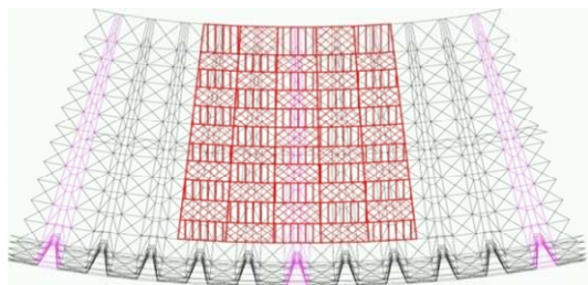
Fig. 18 Section example
