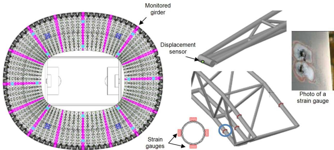
Fig.17 Monitoring system – localization of sensors
