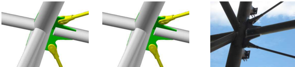
Fig.4 Connection of stiffening to girder – design and realization
