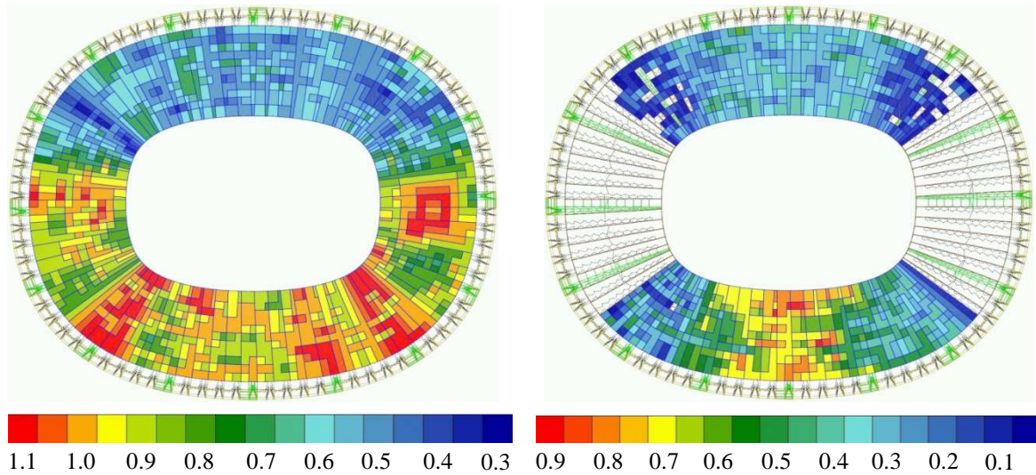
Fig. 20 Estimated snow by evolutionary algorithm for given reference load.
