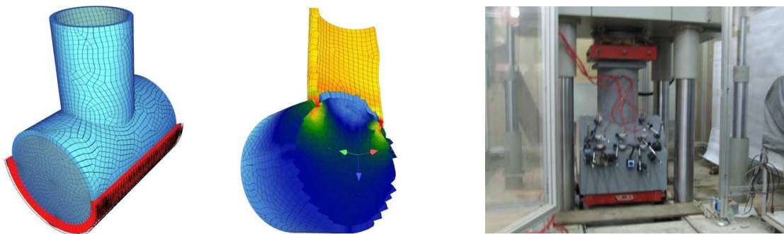
Fig.15 FEA model of the support and stress concentration Fig.16 Laboratory tests of a real scale model
