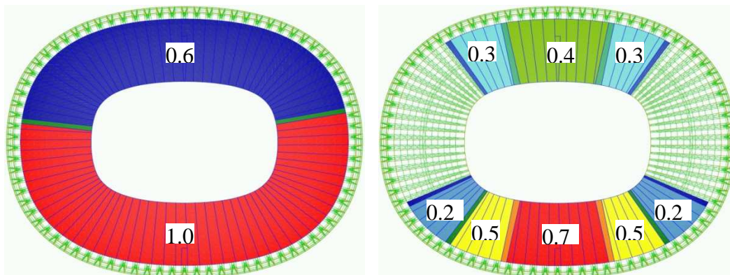
Fig. 19 Reference snow load in numerical
