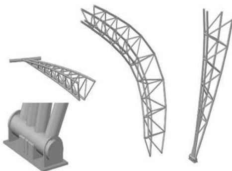
Fig.3 Geometry of three main parts of a single girder
