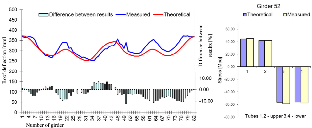
Fig.9 Comparison of numerical and measured results
