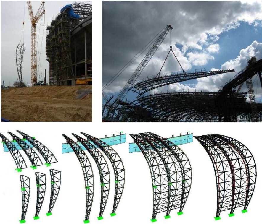
Fig. 8 Installation of facade and roof parts of girder – photos and phases in numerical environment
