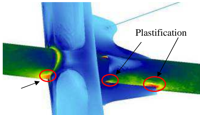
Fig.12 Visualisation of the node with marked places where steel exceeds yield strength
