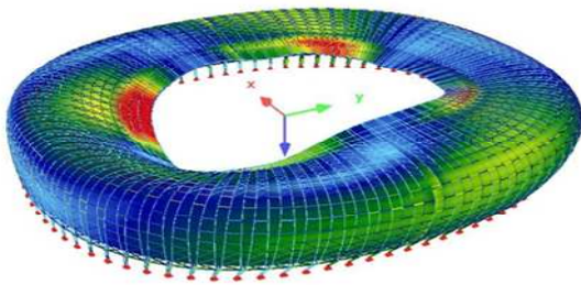
Fig. 6 Roof deformation caused by a north wind
