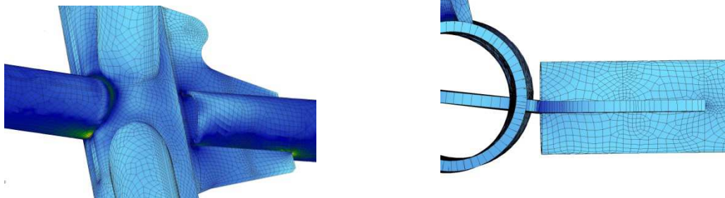
Fig.11 Visualisation of the analysed node with a deformed plate
