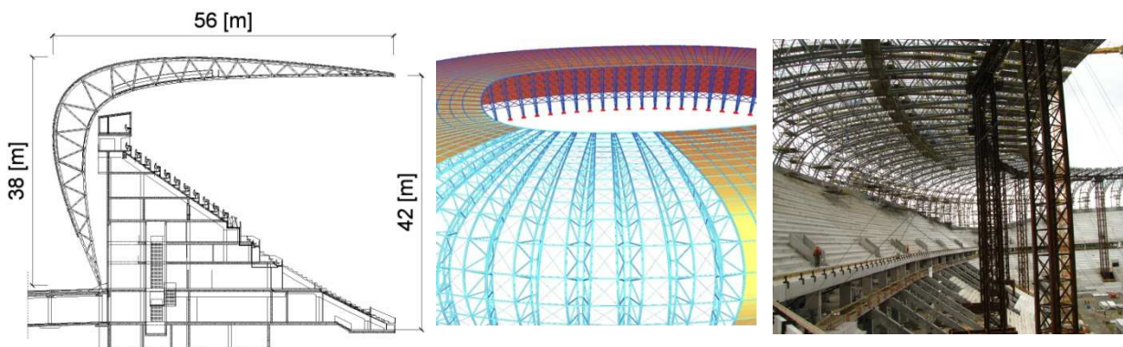
Fig.2 Roof construction. Static model (SOFiSTiK) and photo made 18.08.2010
